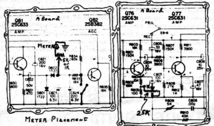
METER Placement POT Placement Refer to Full Schematic of A Board
